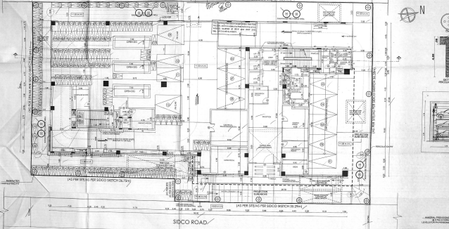
SITE CUM STILT FLOOR (PART) / GROUND FLOOR (PART) PLAN
